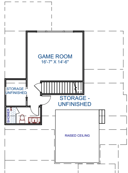
Third Floor
